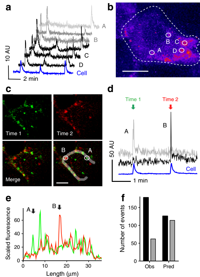
Fig. 3 Secretory events show distinct spatial patterns within a beta cell. (a) Traces of fluorescence intensity in ROIs placed around individual secretory sites during high glucose condition. At some sites secretion occurred repeatedly (black traces), while at others it only occurred once (grey traces); AU, arbitrary units. (b) Temporal stack (13 min 20 s) of confocal images ( n=536 ) of a cell showing the sum of granule secretion during sustained stimulation with high glucose. Fluorescence intensity is highest where more secretory events occurred (pseudocolour scale). Circles denote ROIs for the traces shown in (a). (c) Temporal stacks (30 s) of confocal images of a cell showing secretory events during two secretory bursts (first in green [Time 1], second in red [Time 2]). Scale bar, 5 \mu\text{m} (b, c). (d) Traces of fluorescence intensity in ROIs placed around the individual secretory sites shown in (c). (e) Line scans along the cell membrane outline in (c) showing the profile of fluorescence intensity during the first (green) and second secretory burst (red). Secretory events did not recur at sites A and B (ROIs shown in [c]). (f) Quantification of recurrence of secretory events using the same line scans as those in (e). Bars represent values from a contingency table (black and grey bars for repeated and not repeated events, respectively). The observed number (Obs) of recurring secretory events (black bars) was higher than the predicted number (Pred) (Fisher exact test, p<0.01 , n=13 cells, n=4 islets)
