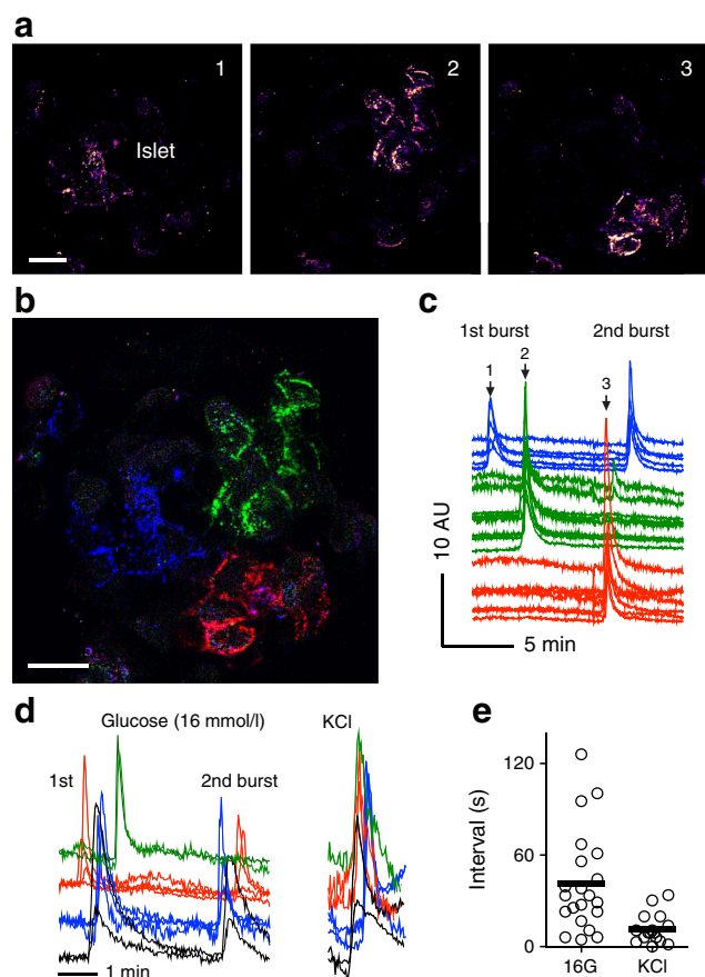
Fig. 5 Islet cells form discrete clusters of synchronised activity. (a) Sequence of temporal stacks (30 s) of confocal images showing secretory events stimulated by high glucose in an intact human islet. (b) Merged image of the temporal stacks shown in (a) , with secretory events colour-coded: blue at time 1; green at time 2 and red at time 3. Three non-overlapping clusters comprising ~10 cells become visible. Scale bars, 20 μm. (c) Traces of secretory responses from cells shown in (b) , with corresponding colours; AU, arbitrary units. Arrows indicate when images in (a) were acquired. (d) Traces of secretory responses from cells in response to high glucose and KCl stimulation (neighbouring cells in a cluster in same colour). The sequence in the activation of cell clusters changes from burst to burst. (e) Quantification of delays in the secretory responses between different clusters in the same islet stimulated with high glucose (16 G) or KCl. Lines represent average values ( n=3 –6 regions per islet, n=3 islets)
