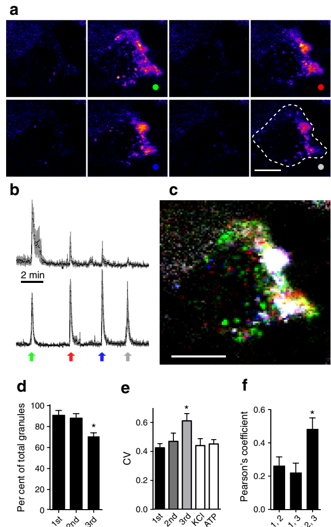
Fig. 4 Secretory events become more localised in subsequent bursts. (a) Sequence of eight temporal stacks (20 s) of confocal images of a cell within an intact islet showing the sum of secretory events before, between and during four secretory bursts (dots) in sustained 16 mmol/l glucose. Scale bar, 5 \mu\text{m} . (b) Average traces of fluorescence intensity in ROIs outside (top) and inside sites of preferential secretion (bottom) ( n=7 ROIs in cell shown in [a]). Peaks of top trace decrease, indicating fewer secretory events. Arrows indicate when images in (a) were taken. (c) Merged image of the temporal stacks of secretory bursts shown in (a). The sums of secretory events per burst are shown in different colours (colours as in a and b). Sites of preferential secretion appear white. Scale bar, 5 \mu\text{m} . (d) The percentage of ROIs with a secretory event (based on recordings as in b) decreases with burst number, reflecting a reduction in secretory events outside regions of preferential secretion ( n=7 cells, *p<0.05 vs 1st burst). (e) CV of cell fluorescence in secretory bursts (30 s temporal stacks) during high glucose, or upon KCl (30 mmol/l) or ATP (100 \mu\text{mol/l} ) stimulation ( n\geq 4 cells, *p<0.05 for comparison between 1st and 3rd bursts during high glucose). (f) Higher Pearson's correlation coefficient shows greater co-localisation of secretory events between pulses 2 and 3 than between pulses 1 and 2 ( *p<0.05 , n=5 cells)
