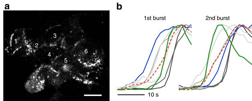
Fig. 6 The sequence of activation of cells within a cluster is not fixed. (a) Temporal stack of confocal images acquired during 30 s showing secretory events in a cell cluster within an intact islet. Numbers indicate different cells within the region. Scale bar, 10 μm. (b) Secretory responses of
