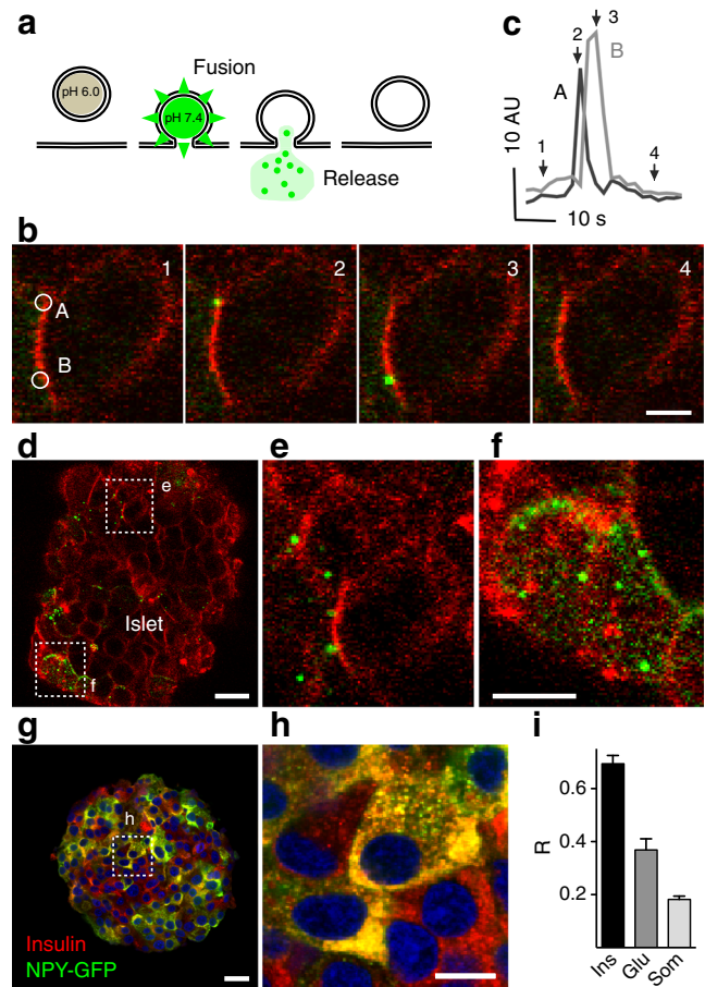
Fig. 1 Imaging insulin granule secretion in intact human islets. (a) The vesicle cargo NPY fused to pHluorin is used to follow insulin granule dynamics in real time. (b) Confocal images showing vesicle secretion (green) at the plasma membrane (red, labelled with di-8-ANEPP) of a cell within an intact human islet, triggered by high glucose, at particular times indicated in (c) . (c) Traces of the changes in fluorescence intensity in ROIs A and B shown in (b) ; AU, arbitrary units. Arrows indicate time points of images in (b) . (d–f) Temporal stack of 20 images (30 s) of a single confocal plane showing high glucose-triggered vesicle secretion in two cells (d) cut transversally by the confocal plane (e) and a cell cut tangentially and exposing its surface (f) . (g, h) Confocal image (g) and higher magnification (h) of an isolated islet immunostained for insulin (red) and GFP (green). (i) Quantification of data in (g) showing Mander's overlap coefficients ( R ), n=5 islets. Ins, insulin; Glu, glucagon; Som, somatostatin. Scale bars, 5 \mu\text{m} ( b, h ), 10 \mu\text{m} ( f ) or 20 \mu\text{m} ( d, g )
