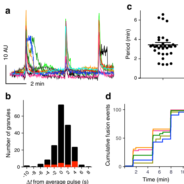
Fig. 2 Secretory events are highly synchronised and generate discrete pulses of secretion in individual beta cells. (a) Traces of fluorescence intensity in ROIs placed around individual secretory sites in a beta cell within an intact islet during sustained stimulation with 16 mmol/l glucose; AU, arbitrary units. Each colour represents an individual site. (b) Histogram showing the difference in time ( \Delta t ) from the start of each secretory event to that of the cell response. Black bars, with IBMX/forskolin; red bars, without IBMX/forskolin. (c) Time between bursts of vesicle secretion (period), n=9 cells, n=3 islet preparations. Periods varied within a cell, from cell to cell, and from preparation to preparation. Line represents the average period \pm SEM. (d) Running sum of the number of secreted vesicles (each coloured trace represents secretory events from a single cell; n=5 cells, normalised to the total number of secretory events). Three bursts of vesicle secretion can be distinguished
